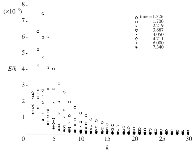
FIGURE 2. E(k)/k versus k for the Wray (1998) DNS data.
