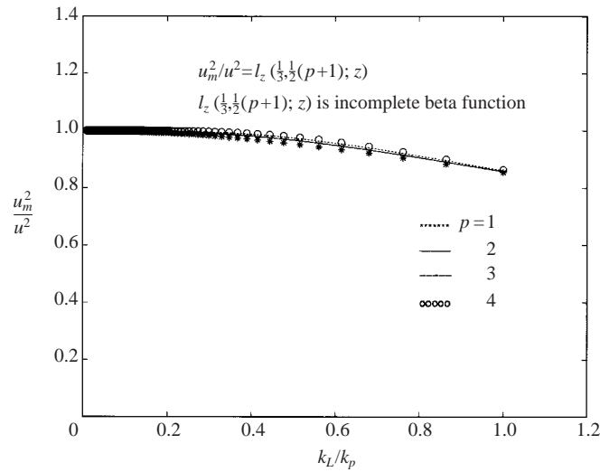
FIGURE 3. Ratio of energy above k_L to total energy versus k_L/k_p .
