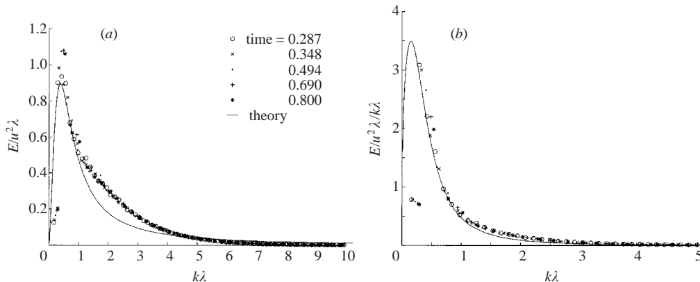
FIGURE 9. (a) E(k)/u^2 \lambda and (b) E(k)/u^2 \lambda / k\lambda versus k\lambda for the de Bruyn Kops & Riley (1998) DNS data.
