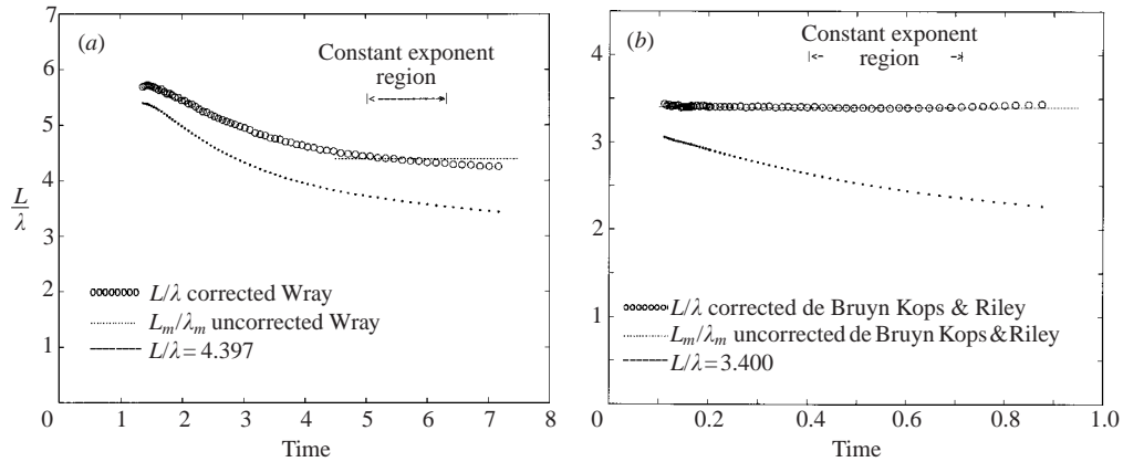
FIGURE 8. Corrected and uncorrected L/\lambda versus t for (a) Wray (1998) data, (b) de Bruyn Kops & Riley (1998) data.
