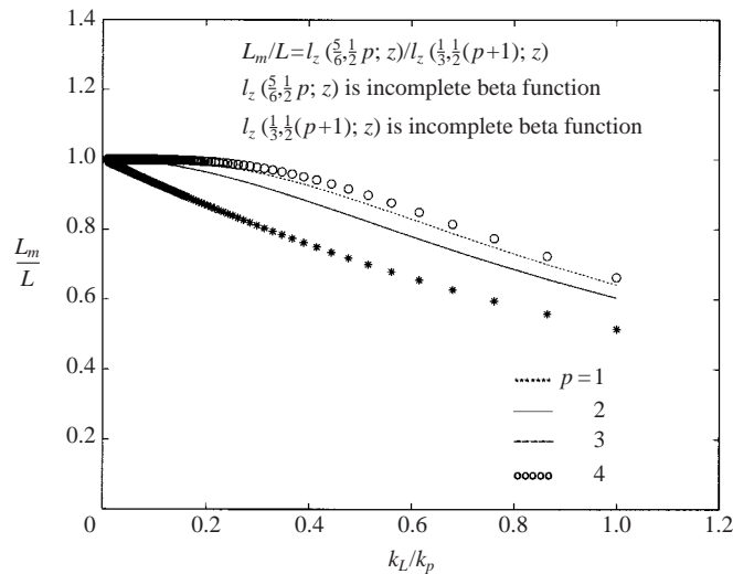
FIGURE 4. Ratio of portion of integral scale above k_L to total integral scale versus k_L/k_p .
