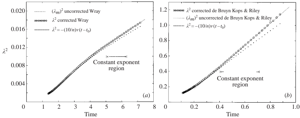
FIGURE 6. Corrected and uncorrected \lambda^2 versus t for (a) Wray (1998) DNS data, (b) de Bruyn Kops & Riley (1998) DNS data.
