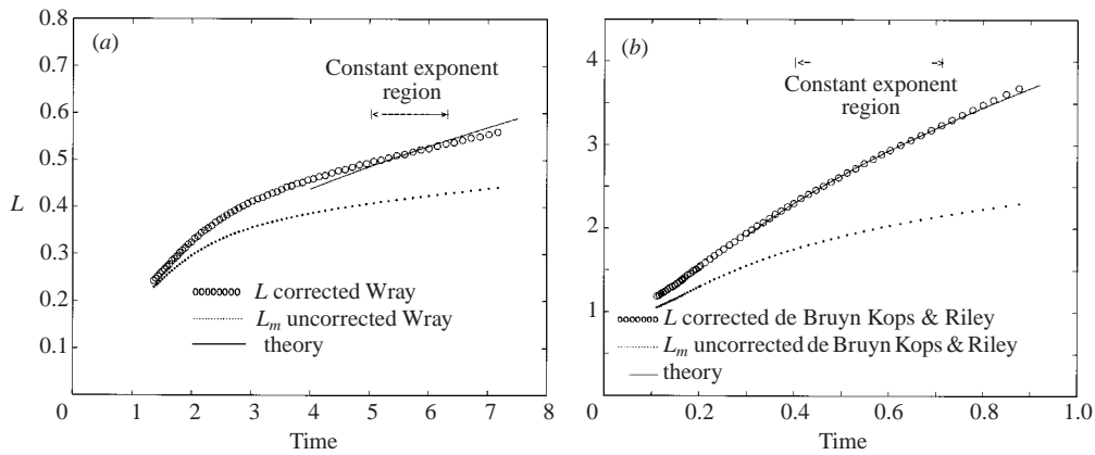
FIGURE 7. Corrected and uncorrected L versus t for (a) Wray (1998) DNS data, (b) de Bruyn Kops & Riley (1998) data.
