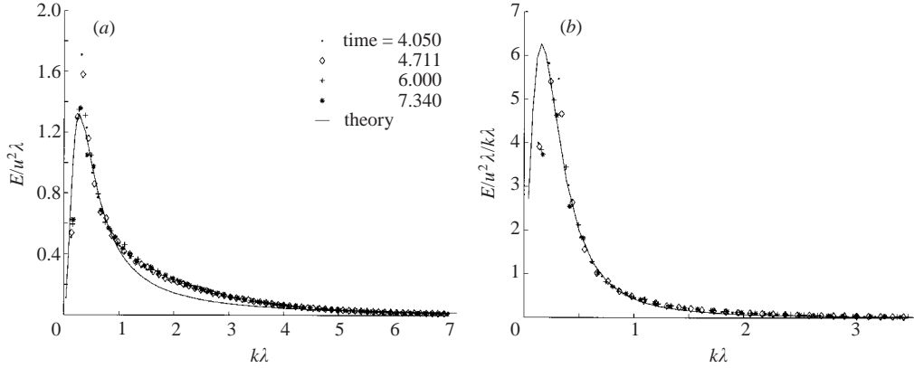
FIGURE 10. (a) E(k)/u^2\lambda and (b) E(k)/u^2\lambda/k\lambda versus k\lambda for the Wray (1998) DNS data.
