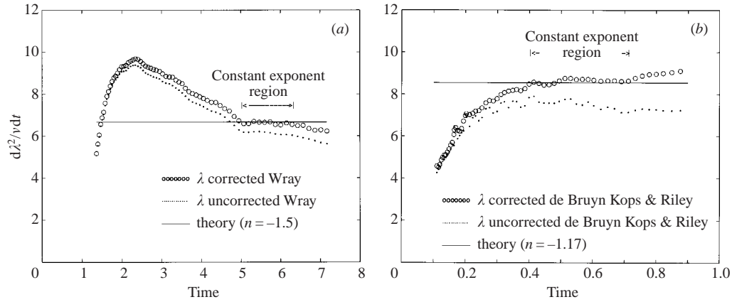
FIGURE 5. Corrected and uncorrected d\lambda^2/vdt versus t for (a) Wray (1998) DNS data, (b) de Bruyn Kops & Riley (1998) DNS data.
