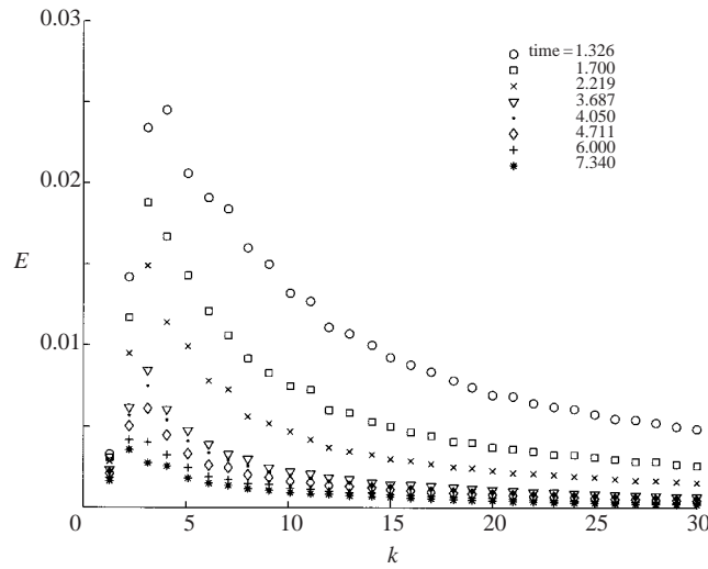
FIGURE 1. E(k) versus k for the Wray (1998) DNS data.
